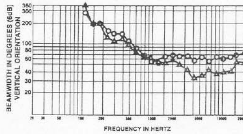
FIGURE 4 — MTH-2.5/64B Beamwidth vs. Frequency
